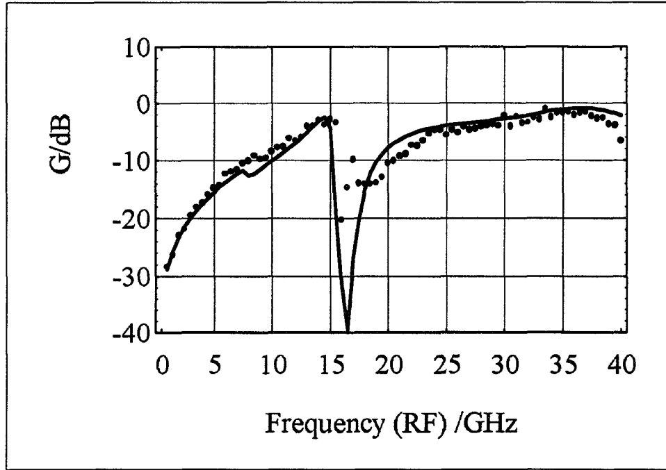
Figure 3: Conversion gain G of the mixer, measured •, nonlinear simulation –, ( V_{GS} = V_t , V_{DS} = 3 V, P_{LO} = 3 dBm, f_{IF} = 100 MHz, R_{IF} = 50 \Omega )
